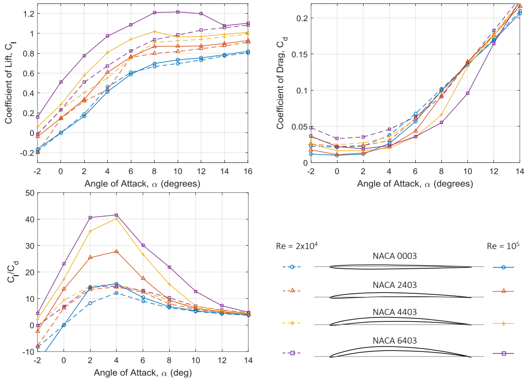
Figure 2.7: Effect of camber on C_l , C_d , and C_l/C_d for NACA Airfoils of 3% t/c at Re = 2 \times 10^4 and 10^5
