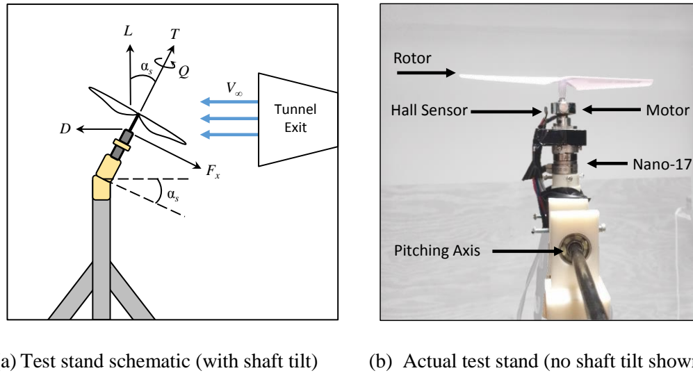
Figure 5.13: Experimental setup used for wind tunnel testing
